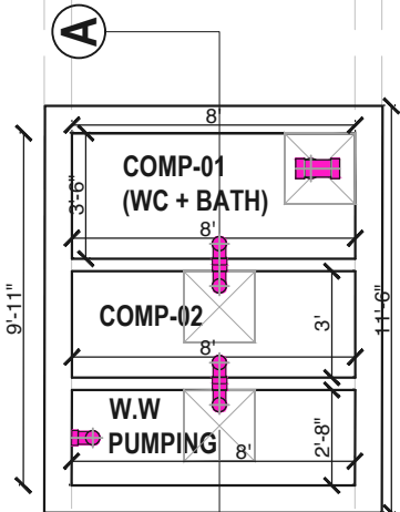
UGT's DETAIL LAYOUT
