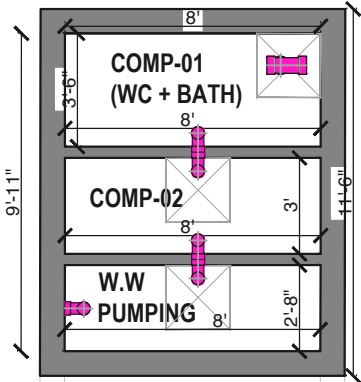
UGT's ARRANGEMENT LAYOUT
