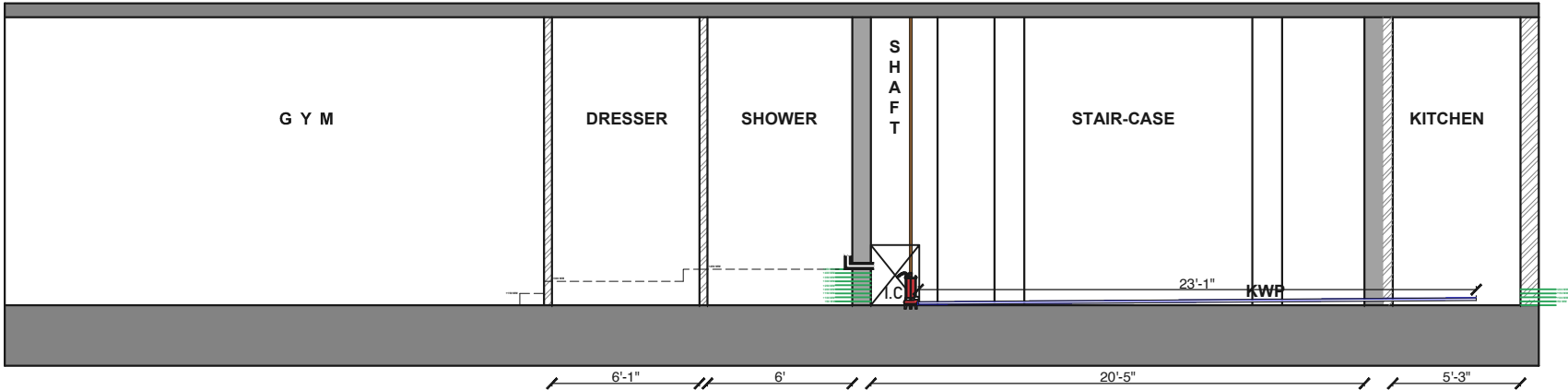
SECTION: S-S
